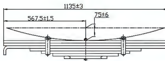
Trailer Leaf Spring
