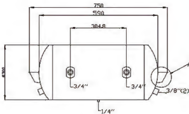
Steel Air Tank
